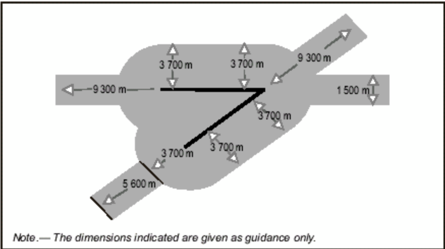
Figure 5-11. Multiple runway laser-beam free flight zone
