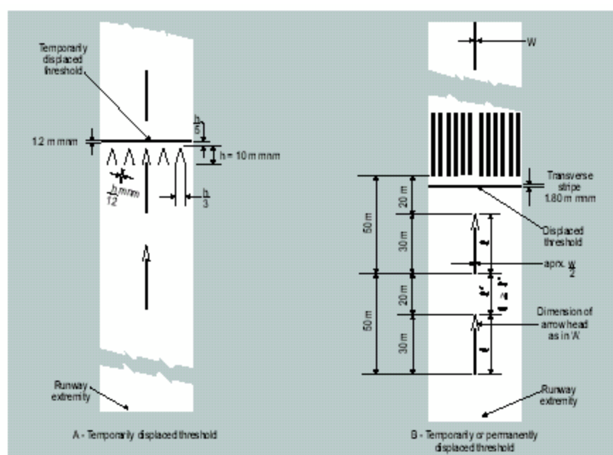
Figure 5-4. Displaced threshold markings
