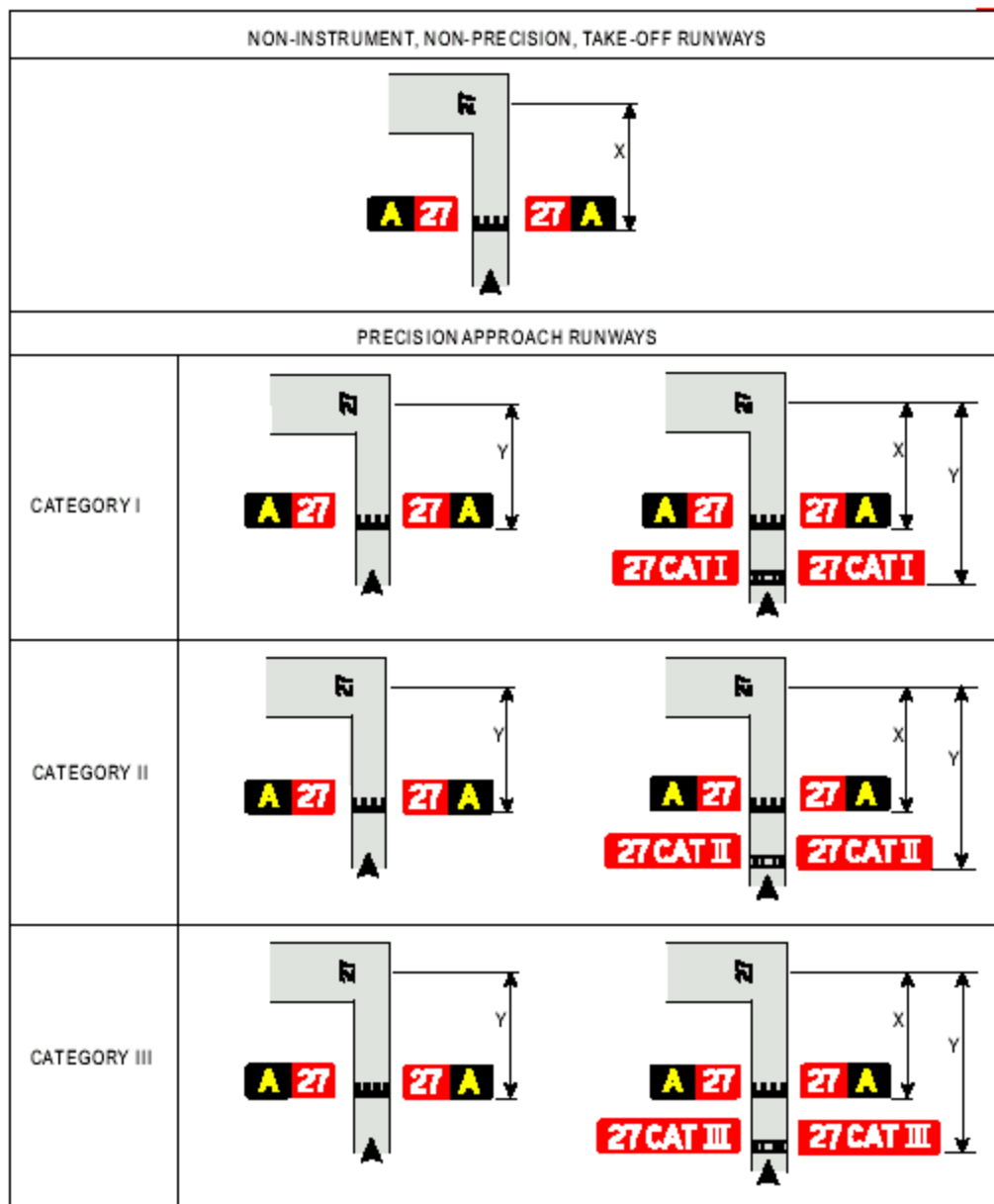
Figure 5-30. Examples of sign positions at taxiway/runway intersections
