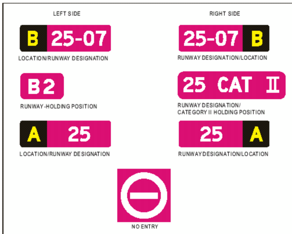
Figure 5-28. Mandatory instruction signs
