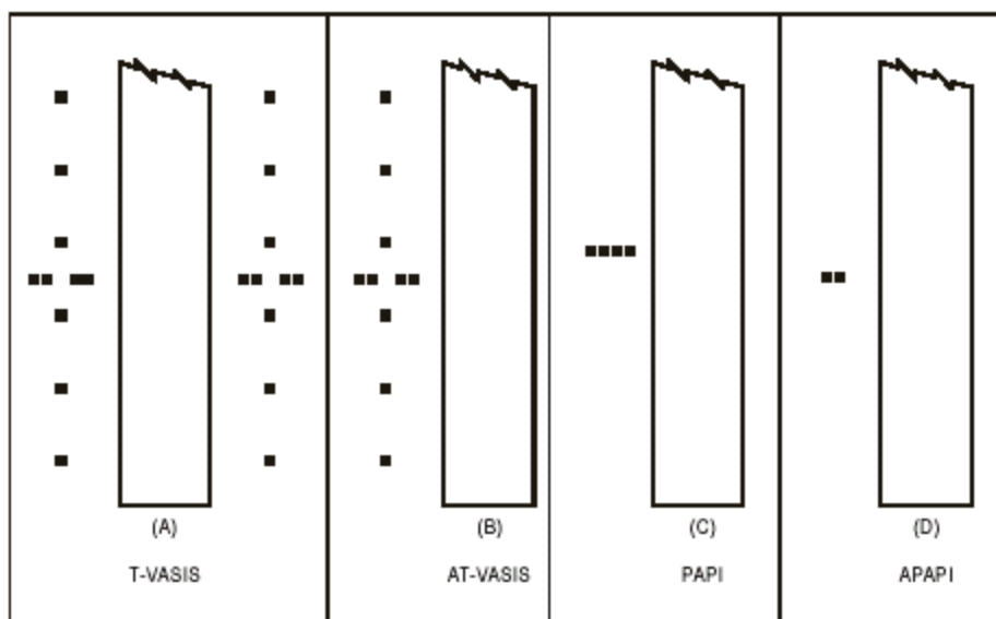
Figure 5-15. Visual approach slope indicator systems
