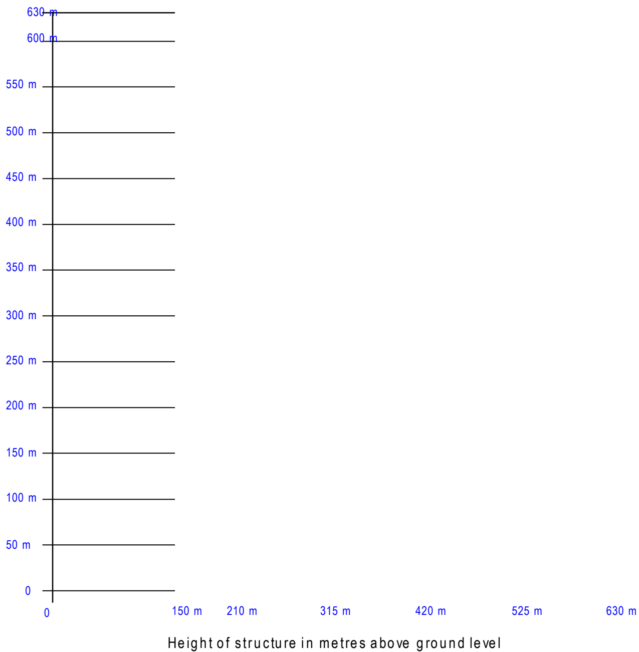
Figure A6-6. High-intensity flashing-white obstacle lighting system, Type A
