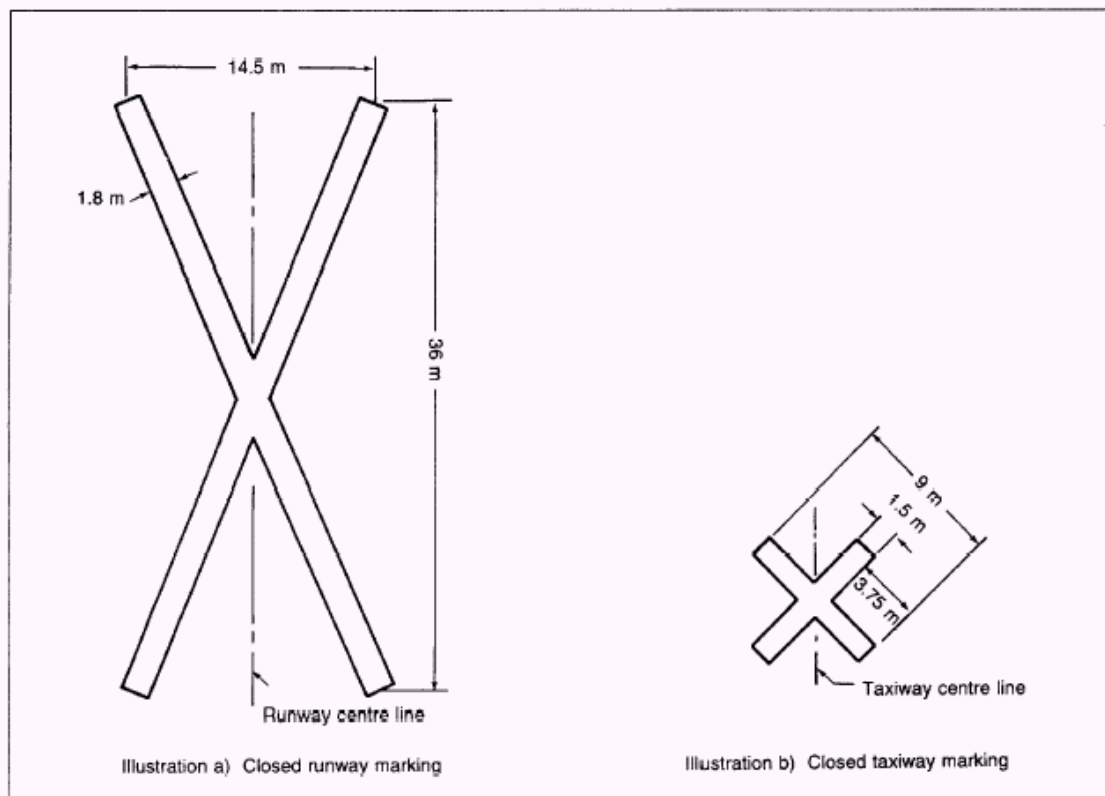
Figure 7-1. Closed runway and taxiway markings
