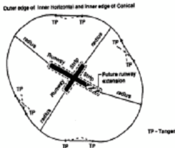
Figure 4.3 Boundary of inner horizontal surface
