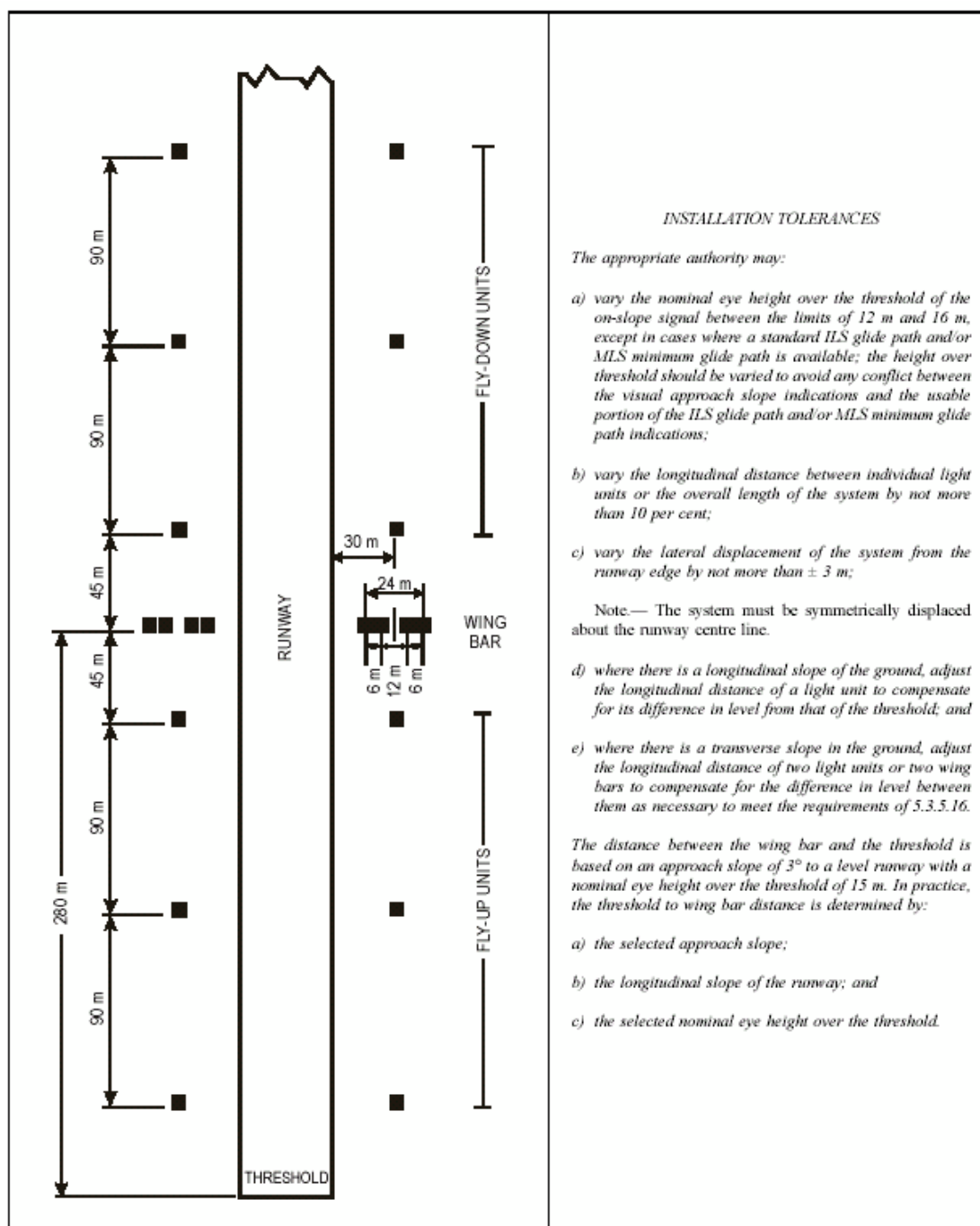
Figure 5-16. Siting of light units for T-VASIS
