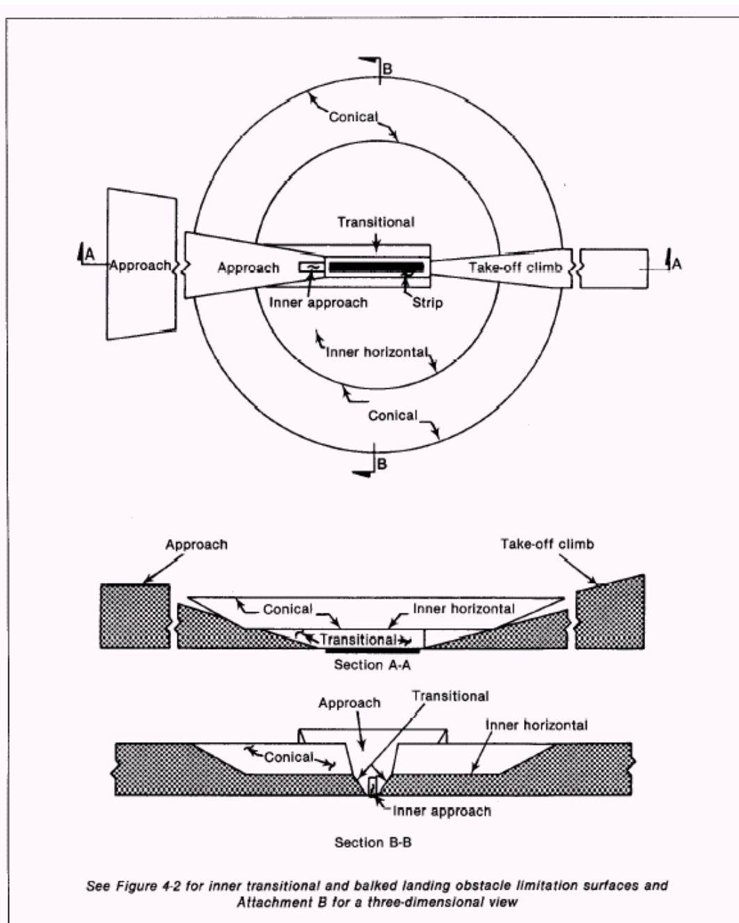
Figure 4-1. Obstacle limitation surfaces
