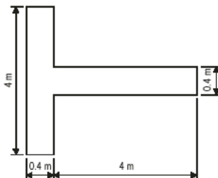
Figure 5-1. Landing direction indicator
