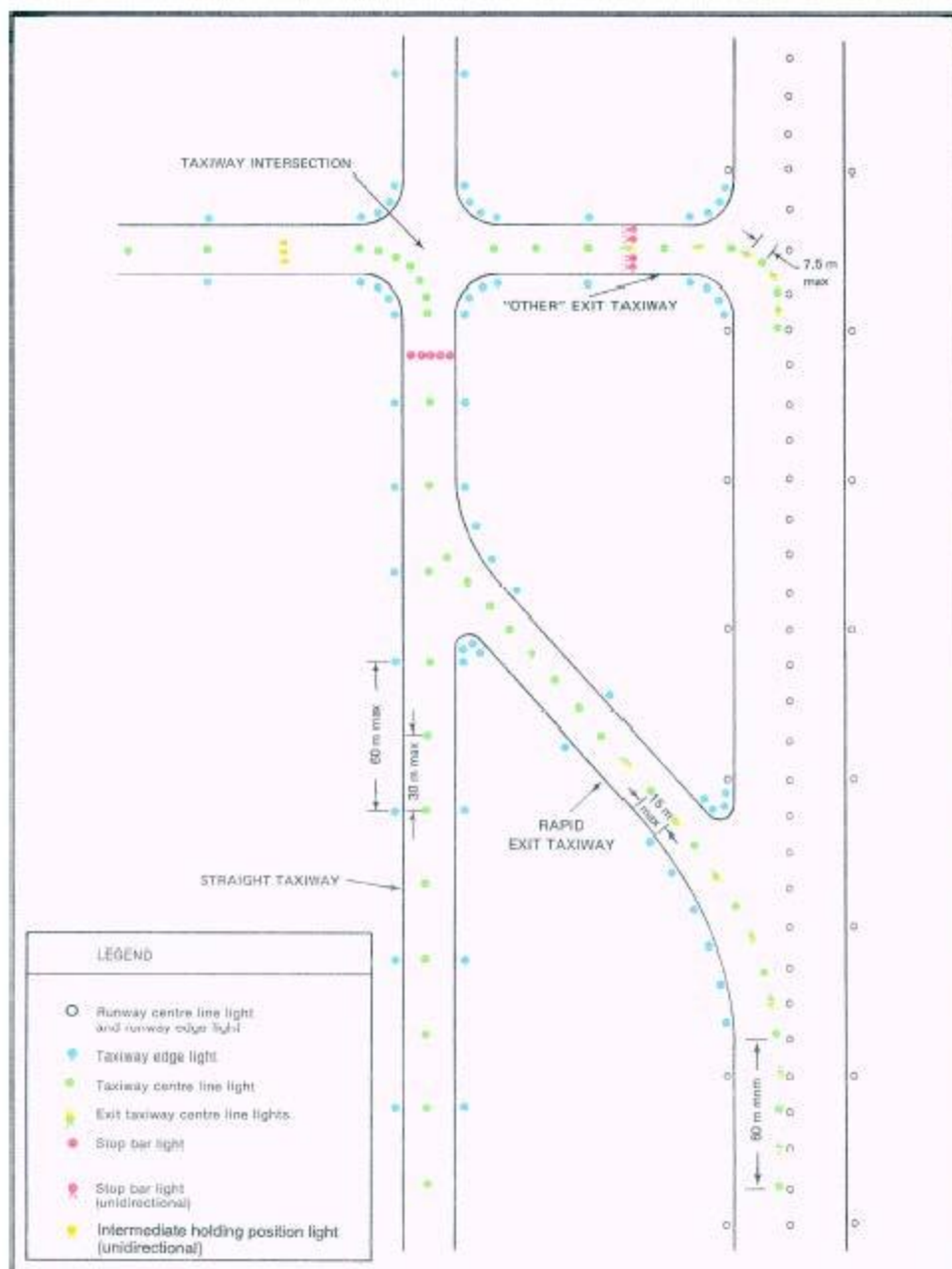
Figure 5-24. Taxiway lighting
