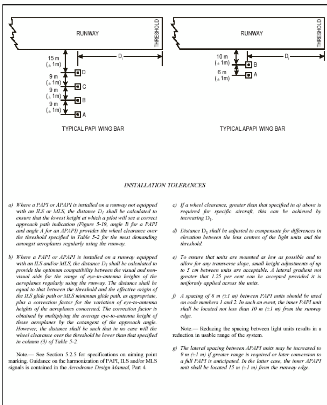
Figure 5-18. Siting of PAPI and APAPI
