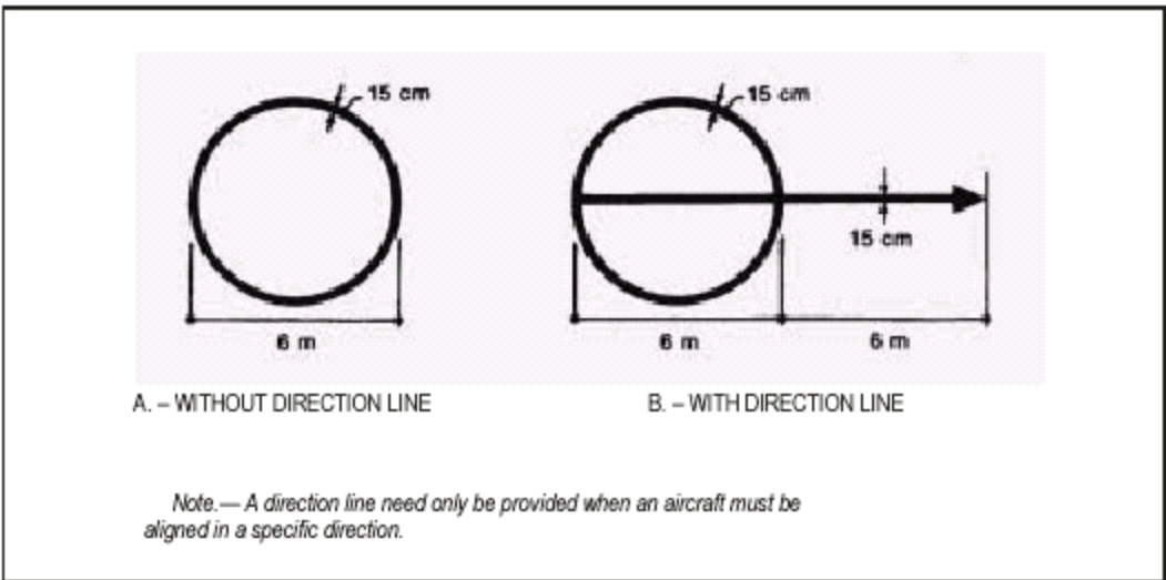
Figure 5-8. VOR aerodrome check-point marking
