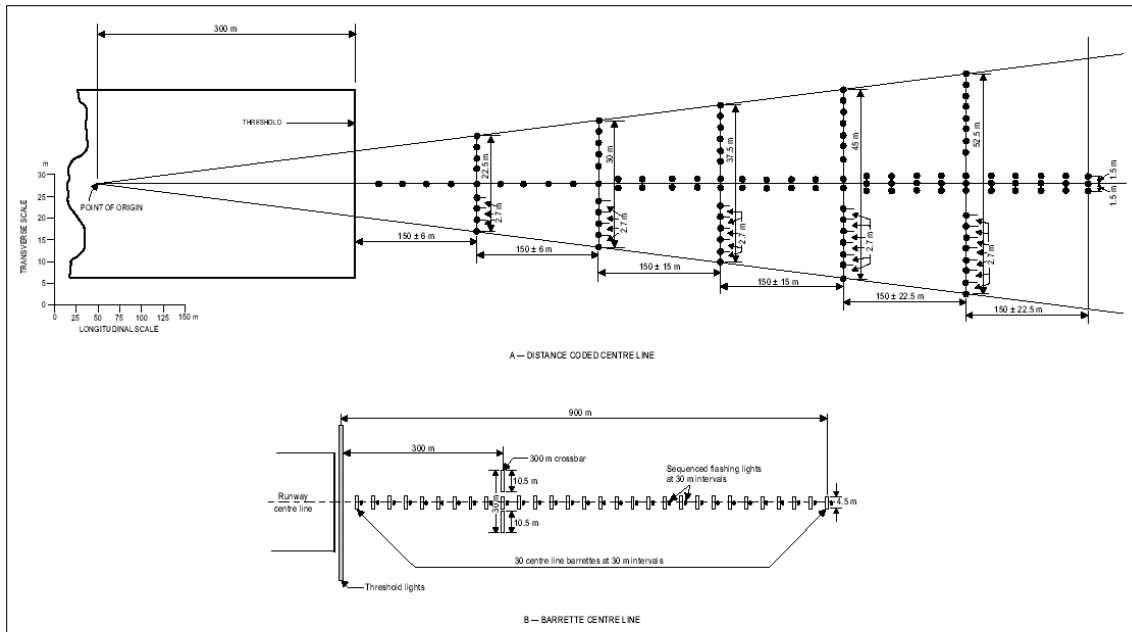
Figure A-6. Precision approach category I lighting systems
