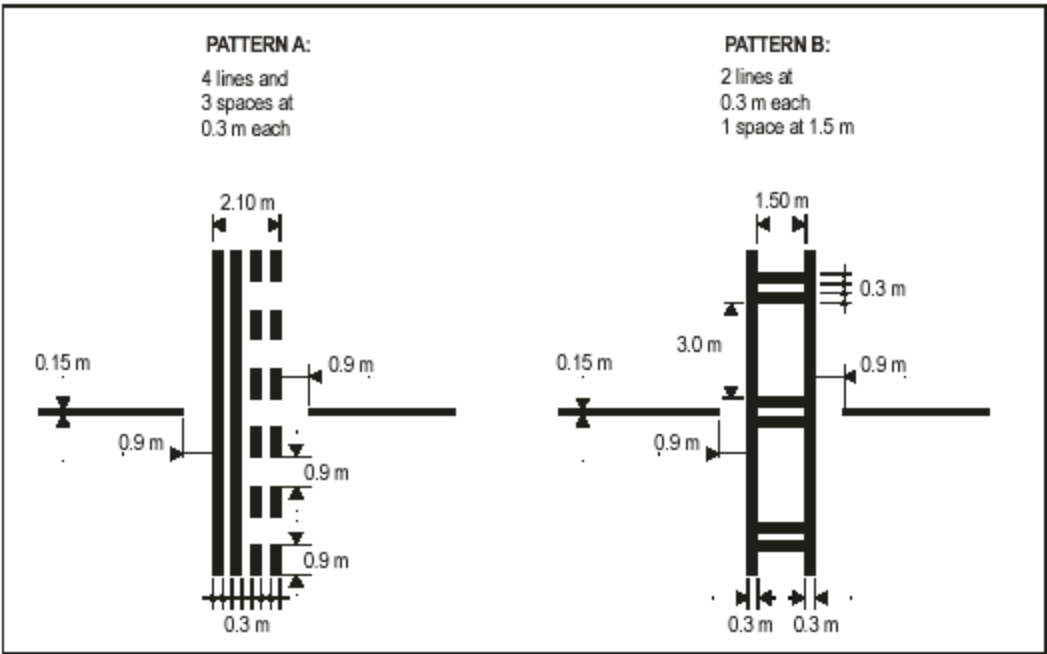
Figure 5-7. Runway-holding position markings
