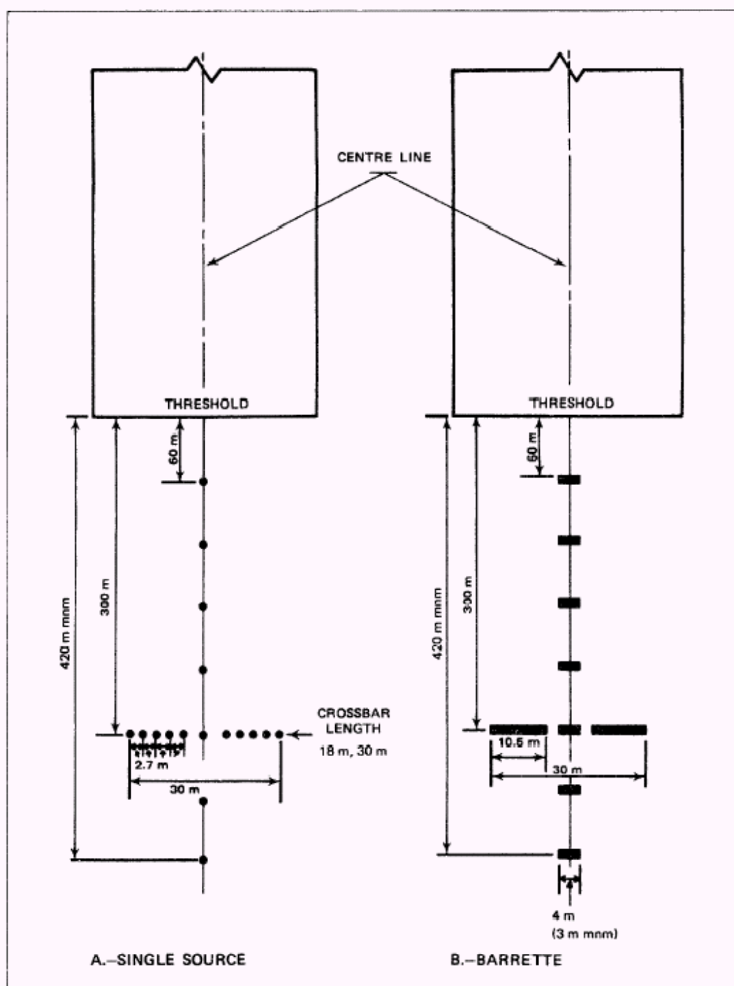
Figure A-5. Simple approach lighting systems
