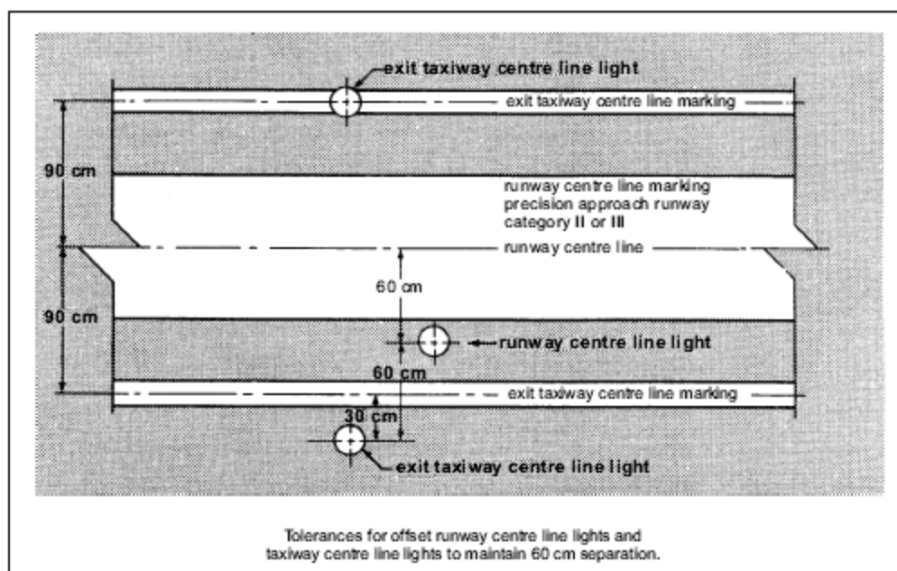
Figure 5-25. Offset runway and taxiway centre line lights
