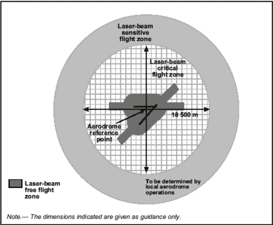
Figure 5-10. Protected flight zones
