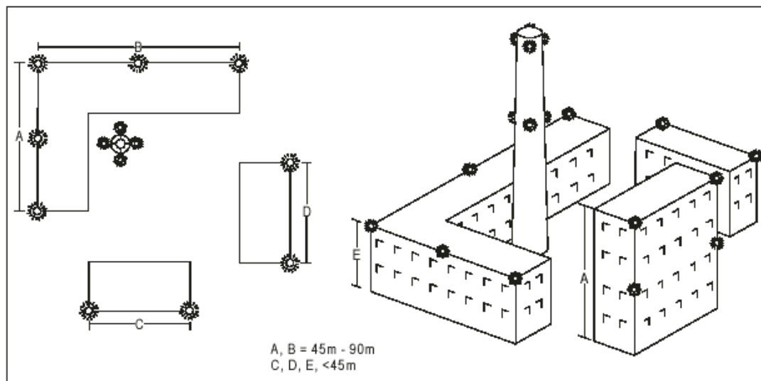
Figure 6-3. Lighting of buildings
