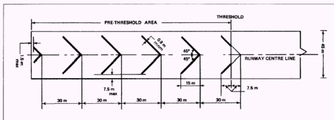
Figure 7-2. Pre-threshold marking
