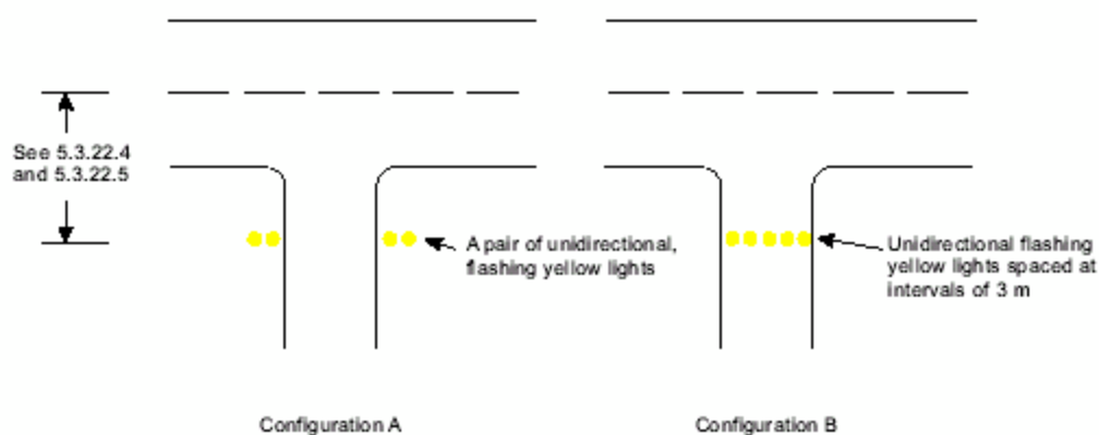
Figure 5-27. Runway guard lights
