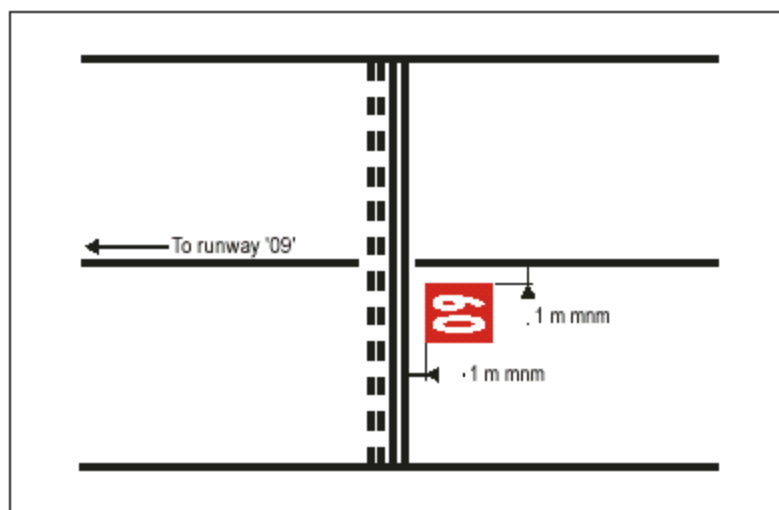
Figure 5-9. Mandatory instruction marking
