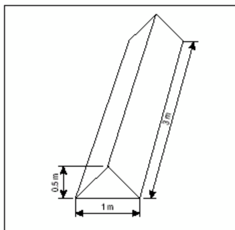
Figure 5-32. Boundary markers
