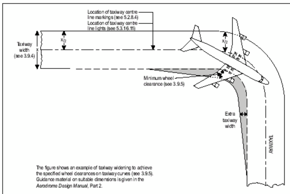
Figure 3-2. Taxiway curve
