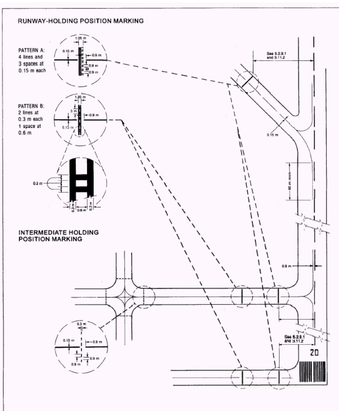
Figure 5-6. Taxiway markings (shown with basic runway markings)
