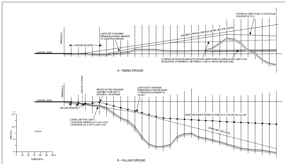
Figure A-7. Vertical installation tolerances
