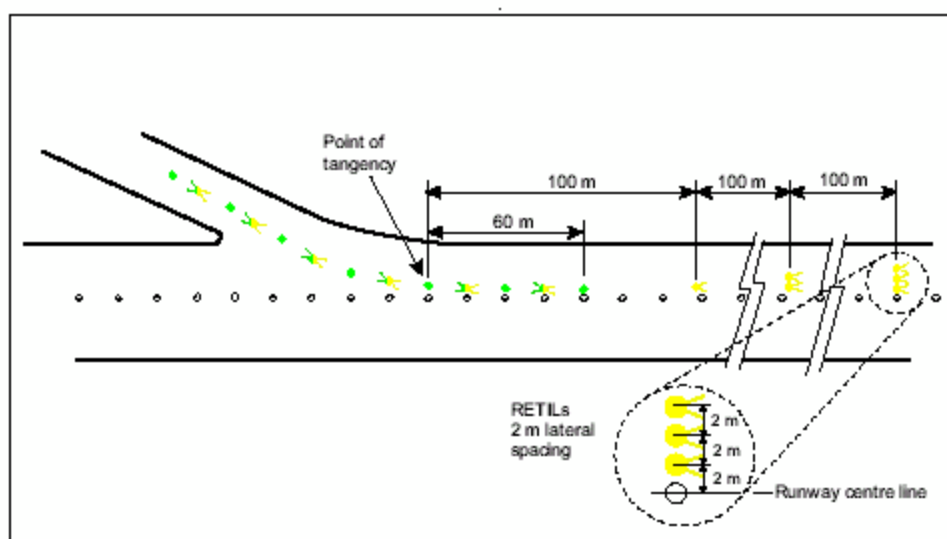
Figure 5-23. Rapid exit taxiway indicator lights (RETILs)
