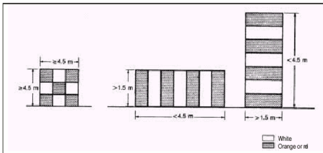
Figure 6-1. Basic marking patterns
