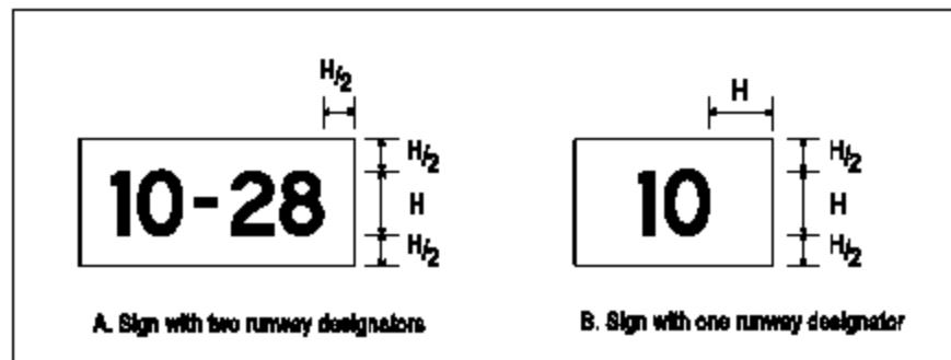
Figure 4.3 Sign dimensions
