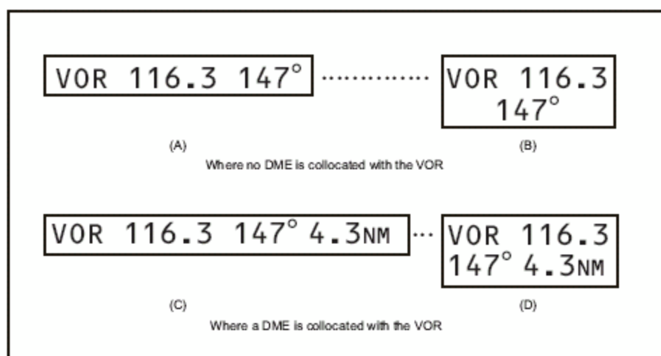
Figure 5-31. VOR aerodrome check-point sign
